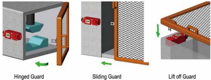
Hinged Guard
