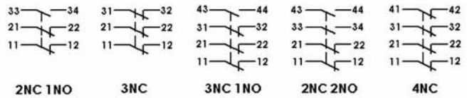
2NC 1NO
